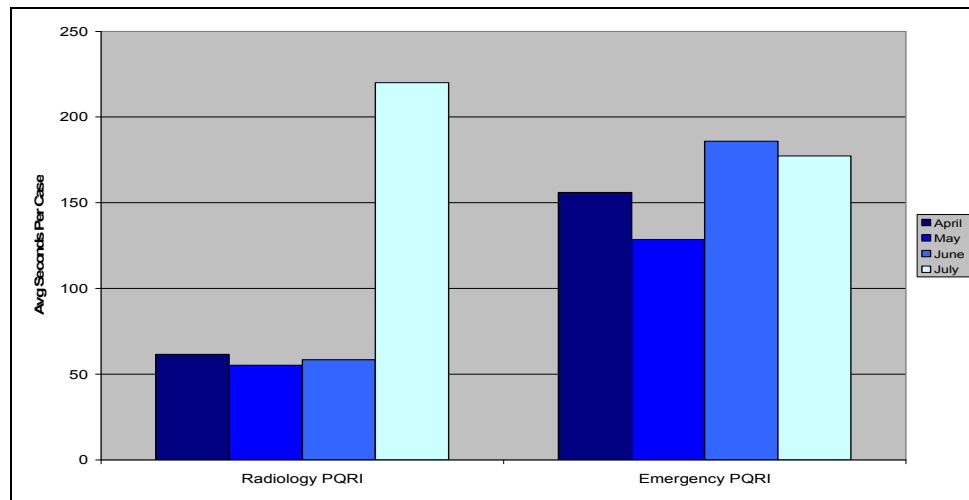
Figure 5: Coder Productivity
